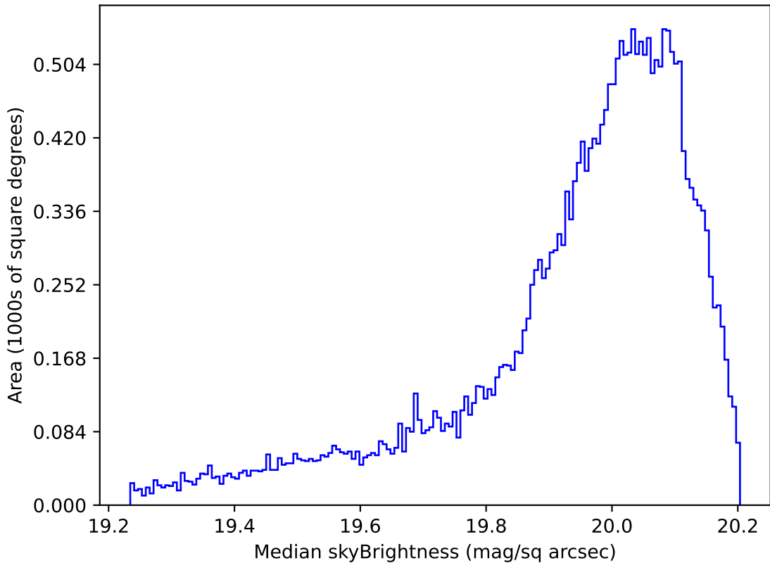
weather_cloudso10v3.4_10yrs All sky i band: Median skyBrightness
