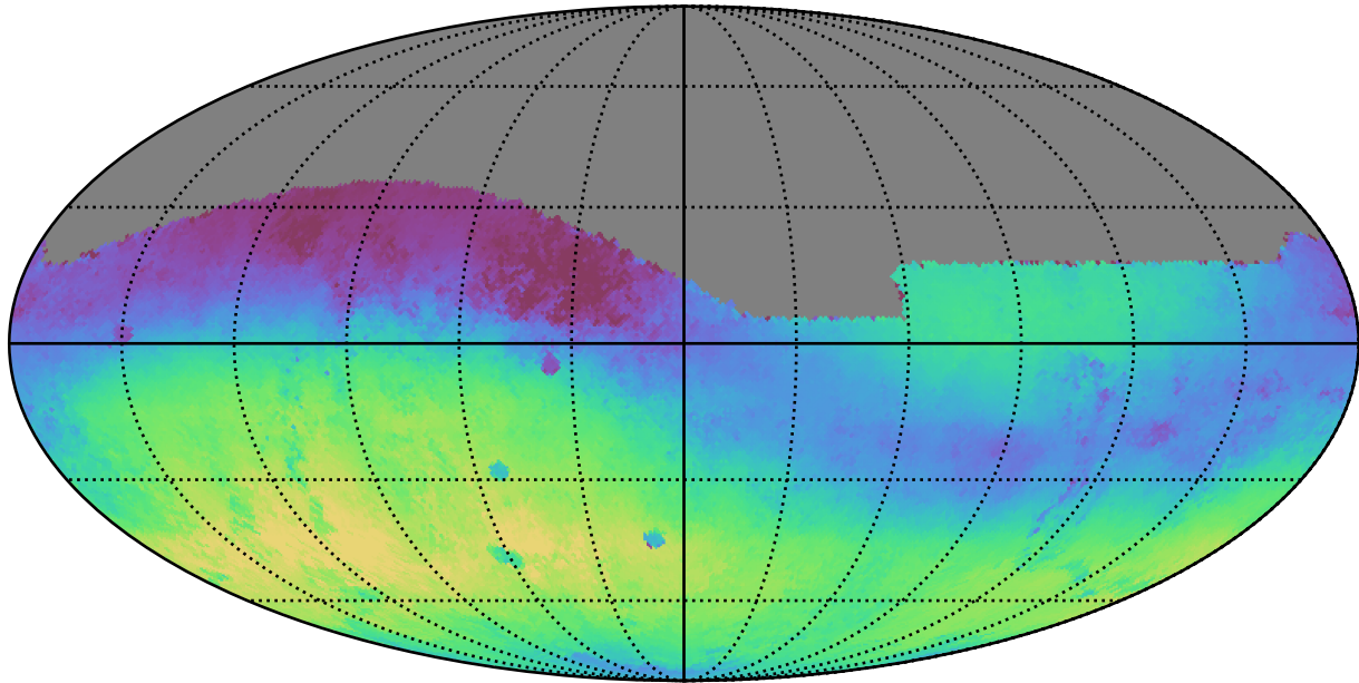
weather_cloudso10v3.4_10yrs All sky g band: Median skyBrightness
