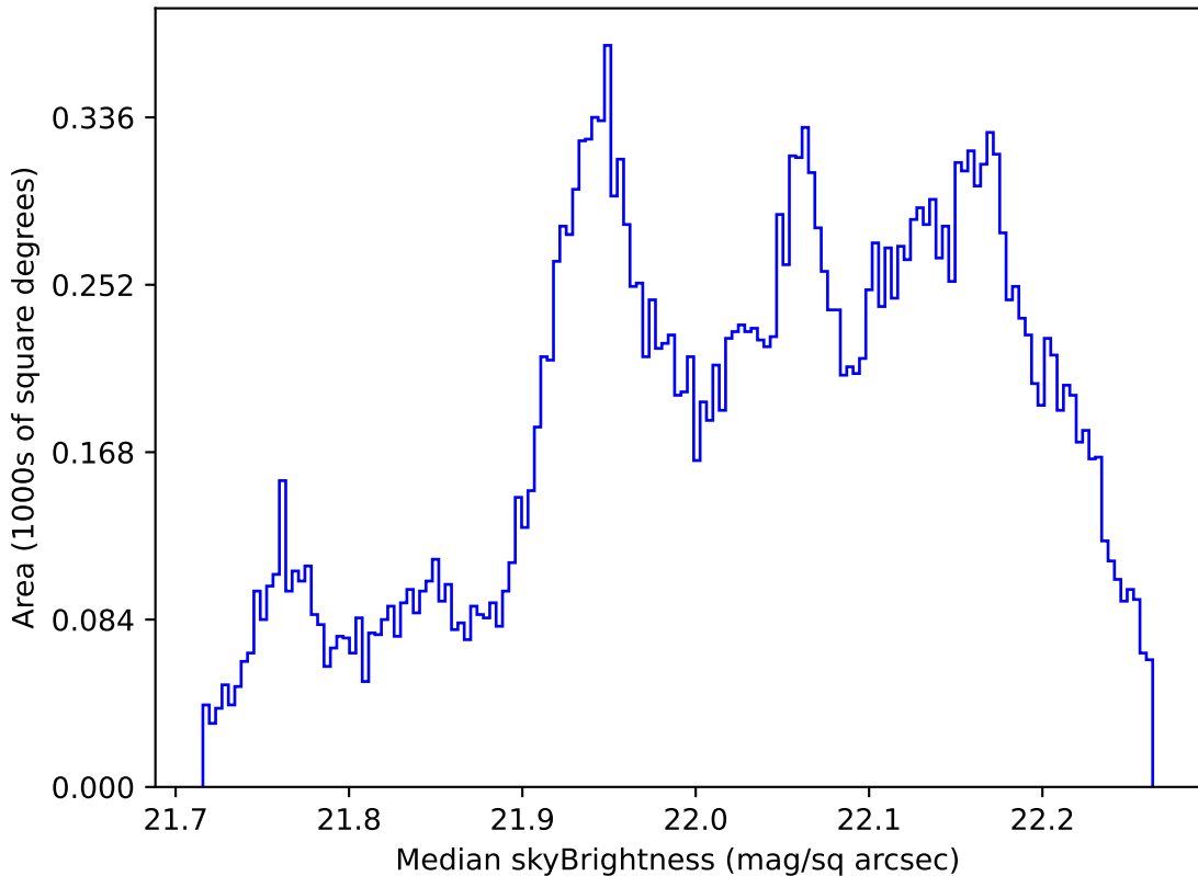
weather_cloudso10v3.4_10yrs All sky g band: Median skyBrightness
