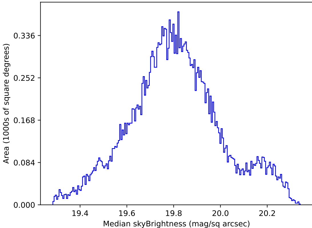
weather_cloudso10v3.4_10yrs All sky all bands: Median skyBrightness
