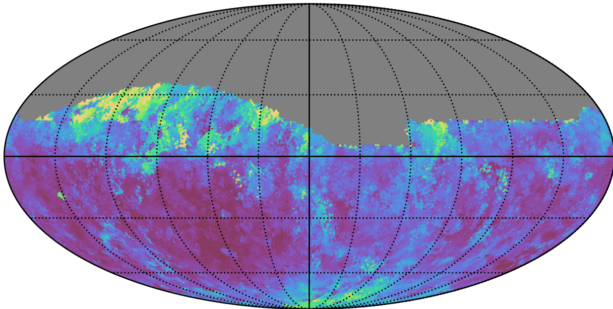
weather_cloudso10v3.4_10yrs Yr 1 z band: Median seeingGeom
