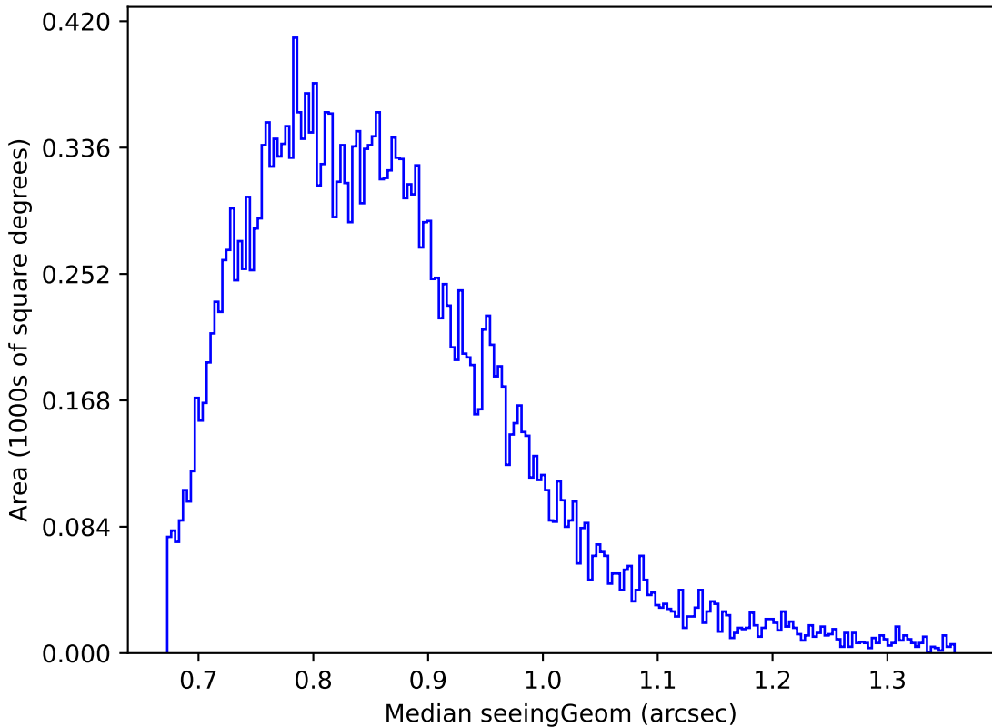
weather_cloudso10v3.4_10yrs Yr 1 z band: Median seeingGeom
