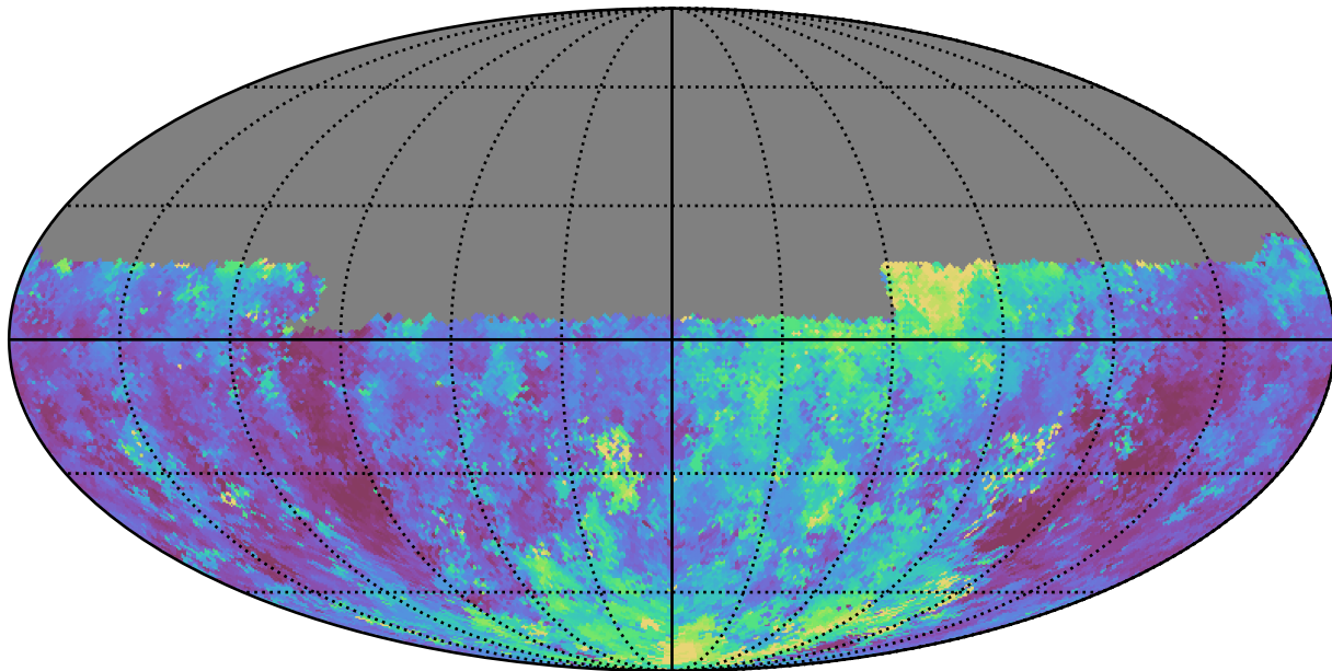
weather_cloudso10v3.4_10yrs Yr 1 u band: Median seeingGeom
