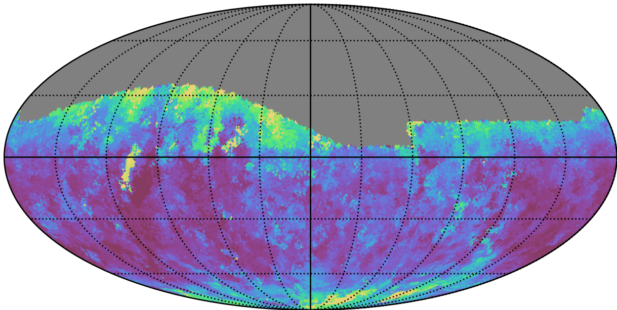
weather_cloudso10v3.4_10yrs Yr 1 r band: Median seeingGeom
