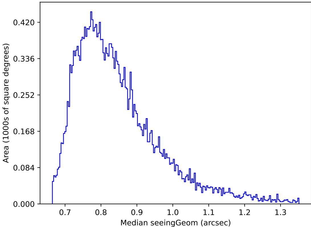
weather_cloudso10v3.4_10yrs Yr 1 i band: Median seeingGeom
