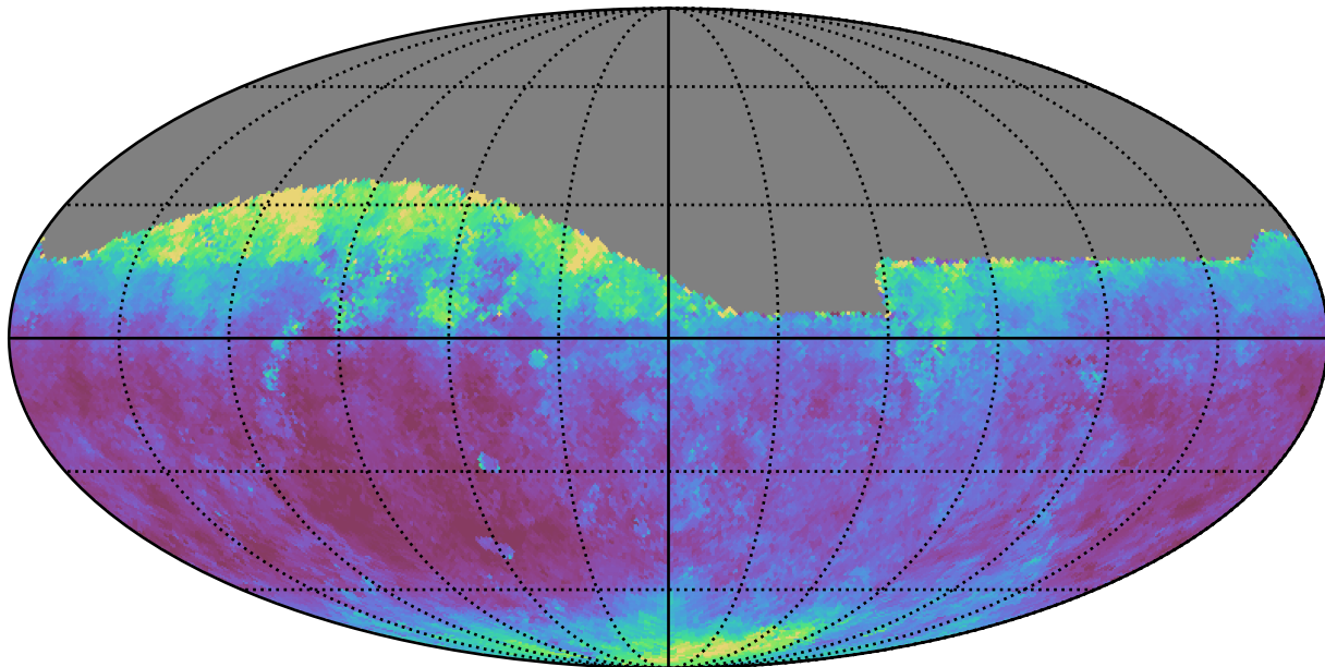
weather_cloudso10v3.4_10yrs Yr 1 all bands: Median seeingGeom
