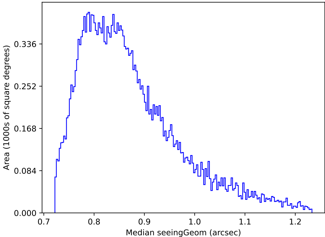
weather_cloudso10v3.4_10yrs Yr 1 all bands: Median seeingGeom
