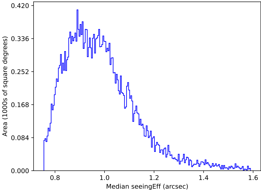
weather_cloudso10v3.4_10yrs Yr 1 z band: Median seeingEff
