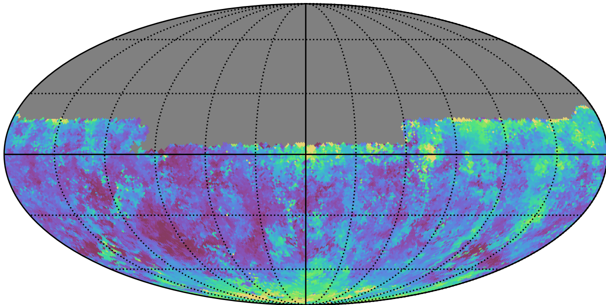
weather_cloudso10v3.4_10yrs Yr 1 y band: Median seeingEff
