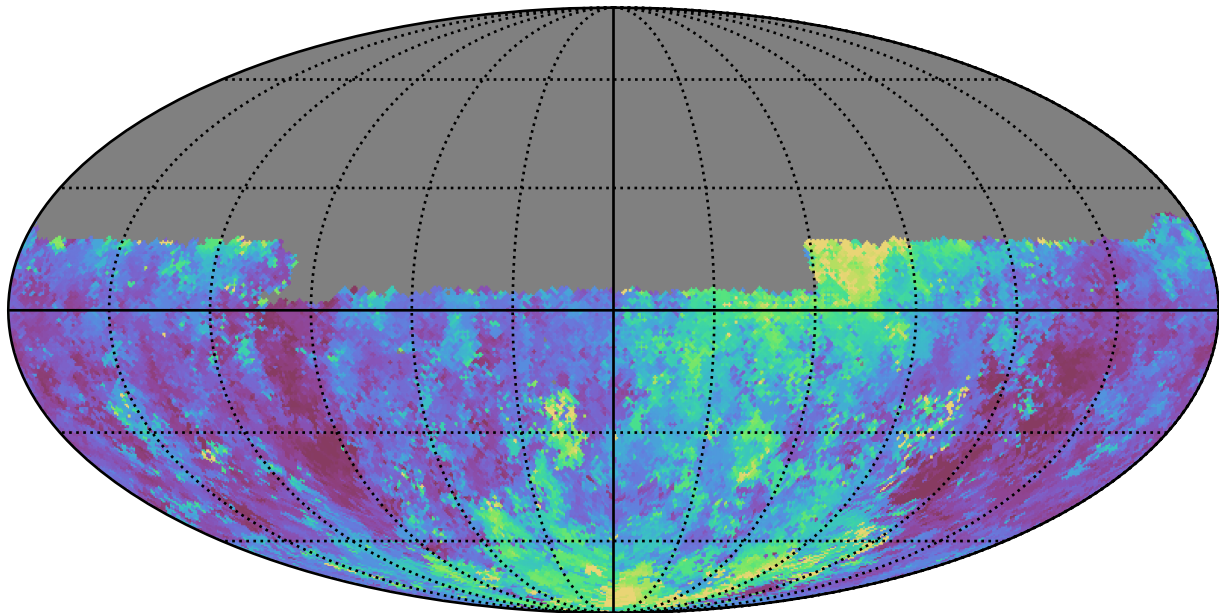
weather_cloudso10v3.4_10yrs Yr 1 u band: Median seeingEff
