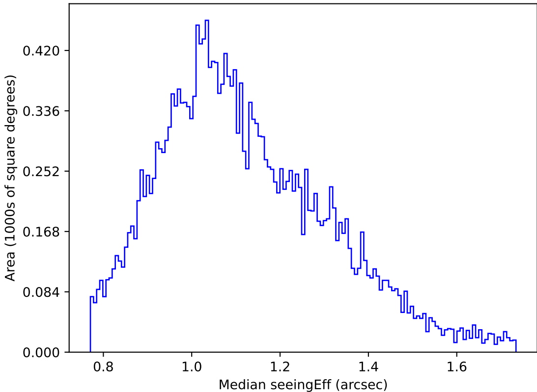
weather_cloudso10v3.4_10yrs Yr 1 u band: Median seeingEff
