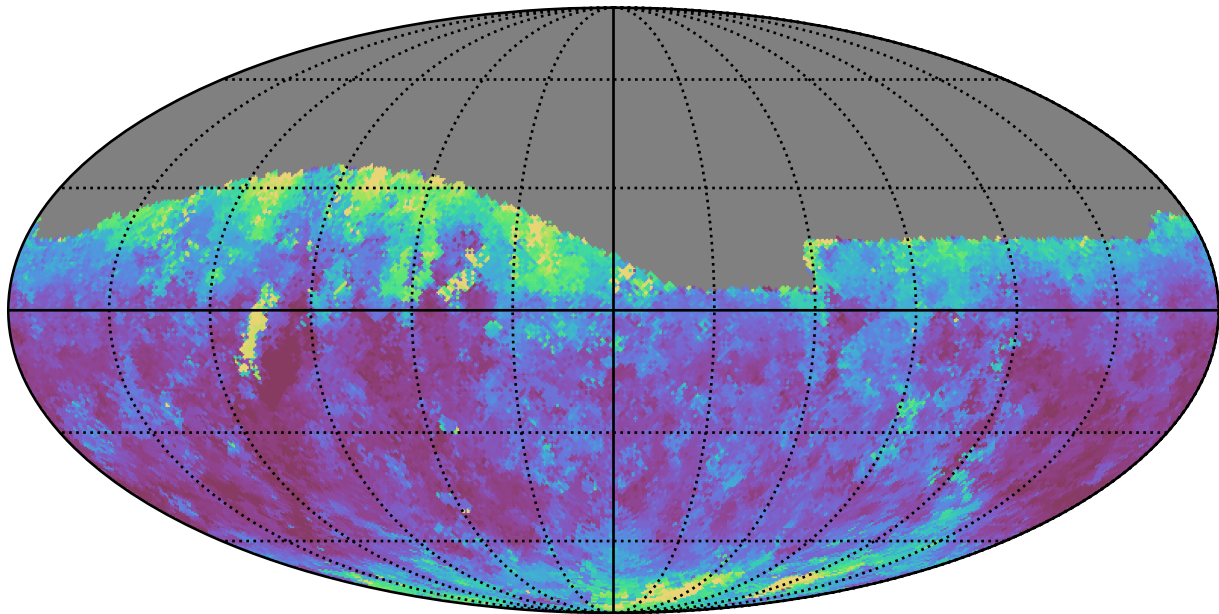
weather_cloudso10v3.4_10yrs Yr 1 r band: Median seeingEff
