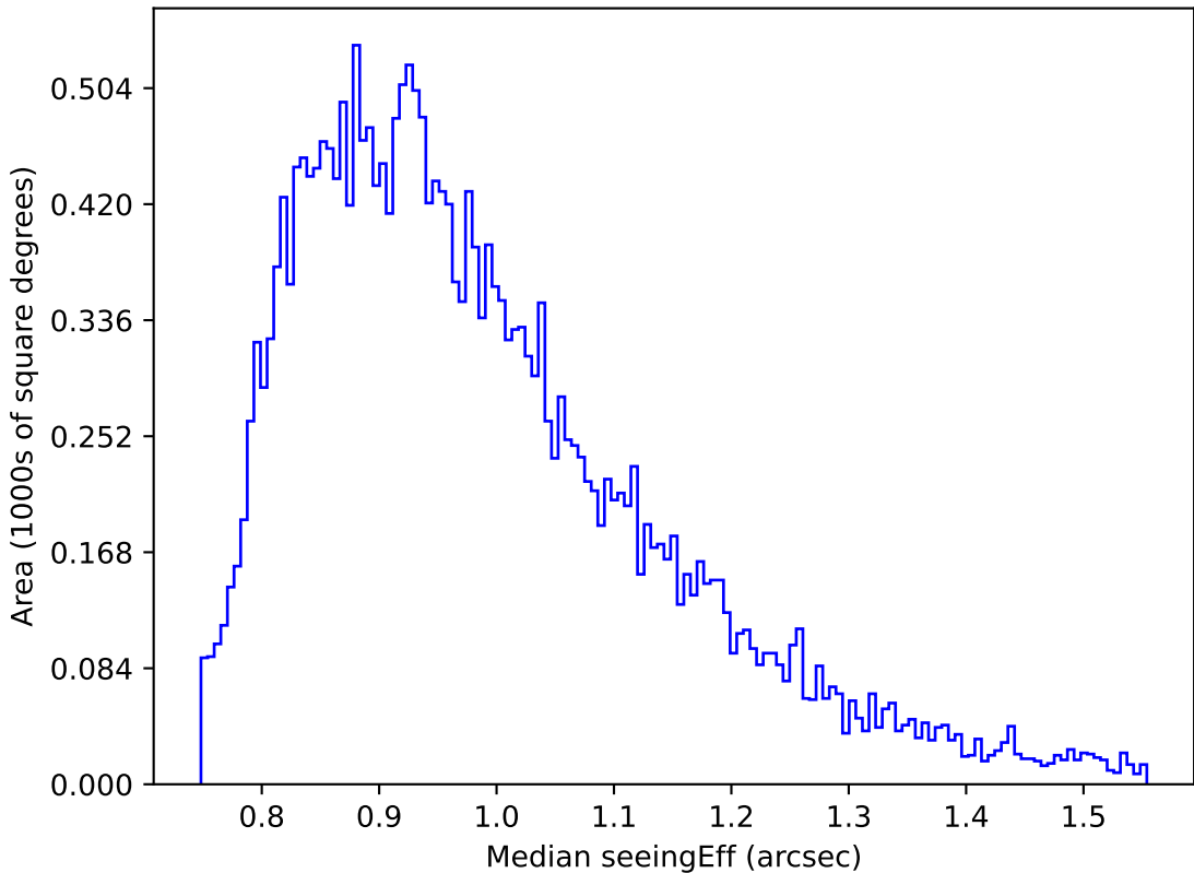
weather_cloudso10v3.4_10yrs Yr 1 r band: Median seeingEff
