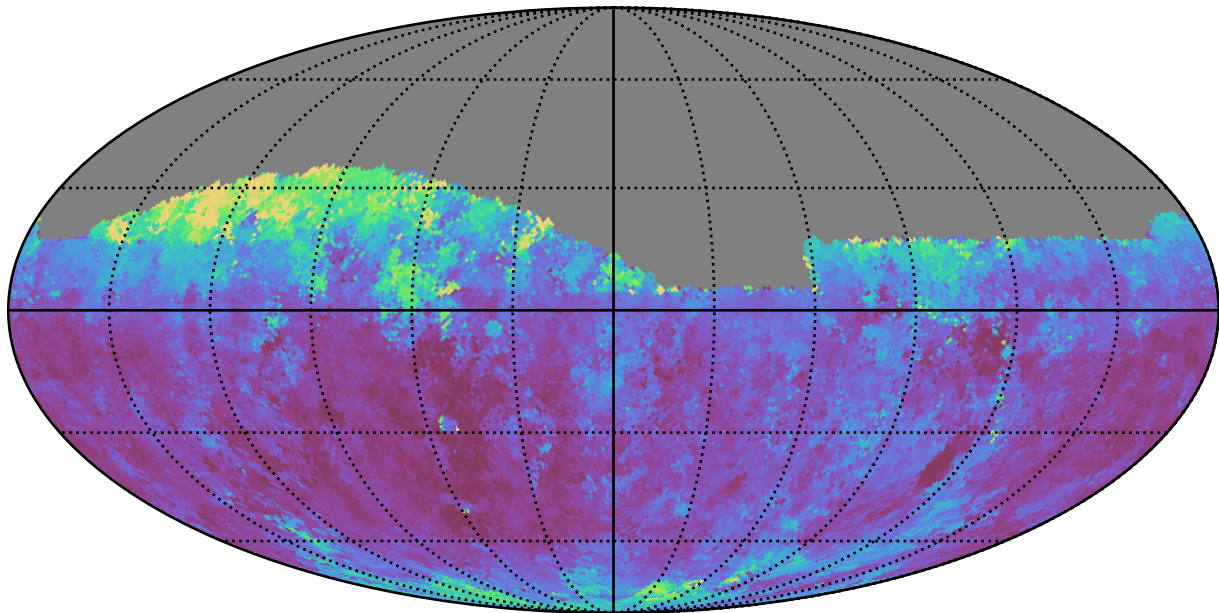
weather_cloudso10v3.4_10yrs Yr 1 i band: Median seeingEff
