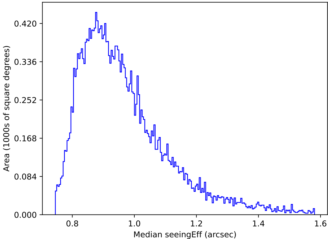
weather_cloudso10v3.4_10yrs Yr 1 i band: Median seeingEff
