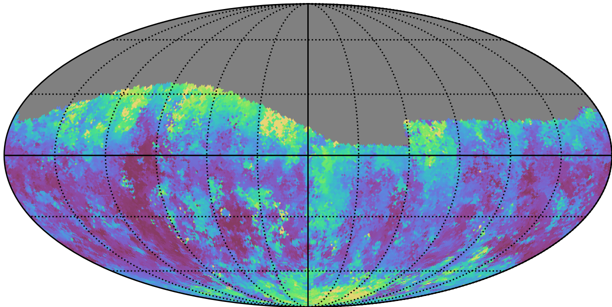
weather_cloudso10v3.4_10yrs Yr 1 g band: Median seeingEff
