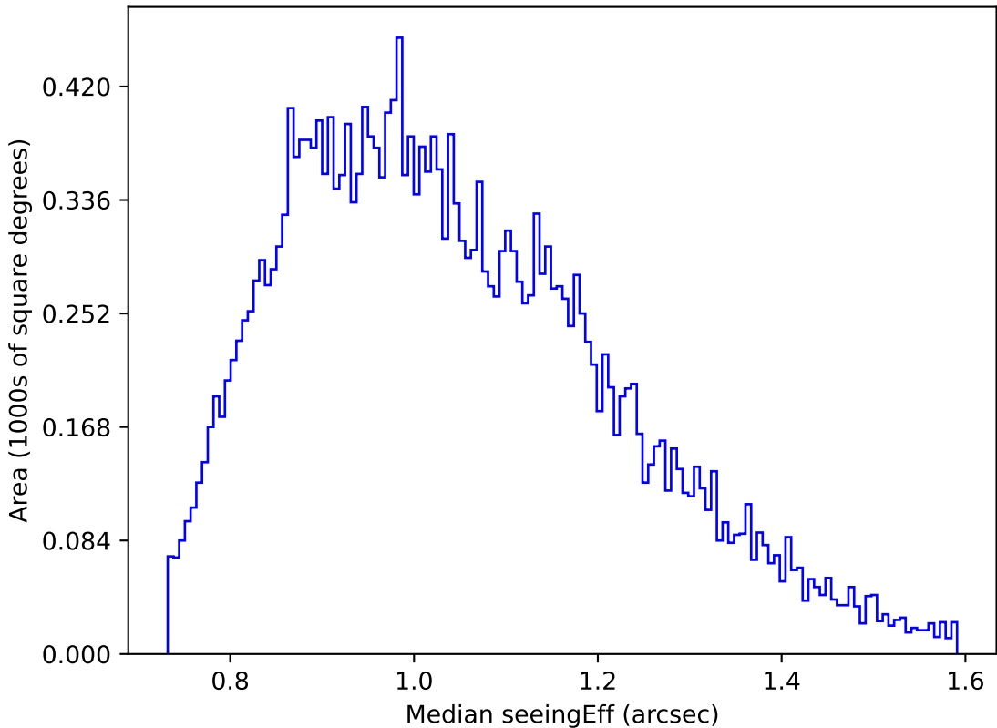
weather_cloudso10v3.4_10yrs Yr 1 g band: Median seeingEff
