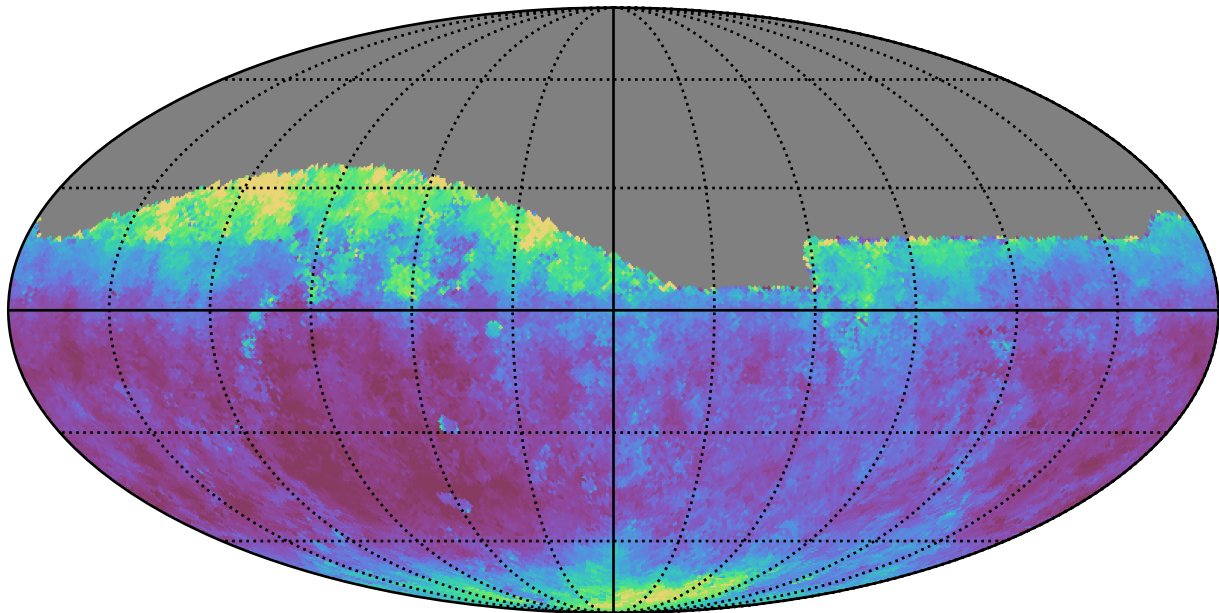
weather_cloudso10v3.4_10yrs Yr 1 all bands: Median seeingEff
