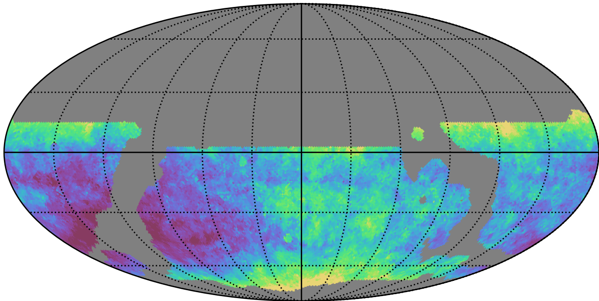
weather_cloudso10v3.4_10yrs WFD z band: Median seeingEff
