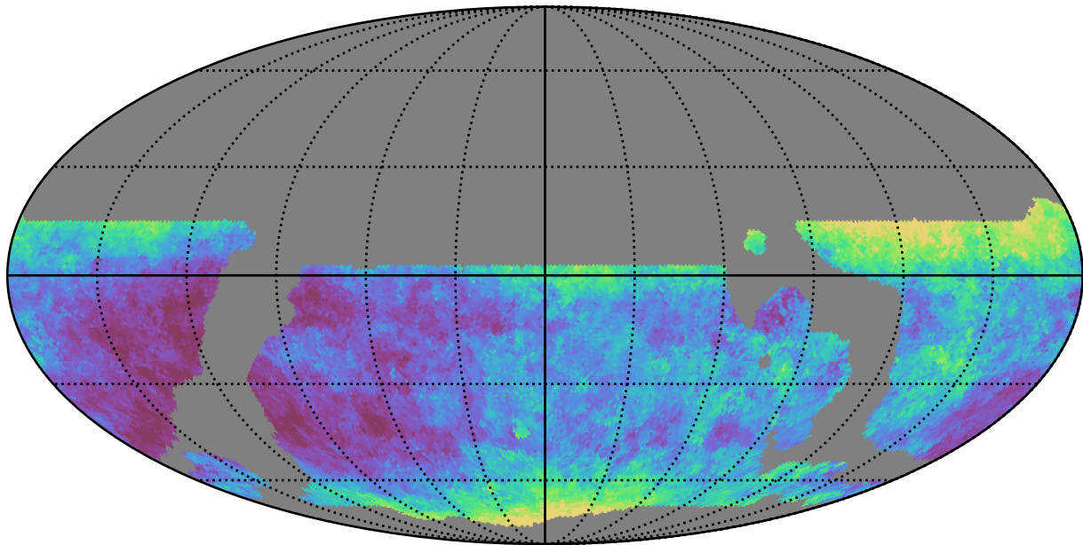
weather_cloudso10v3.4_10yrs WFD y band: Median seeingEff
