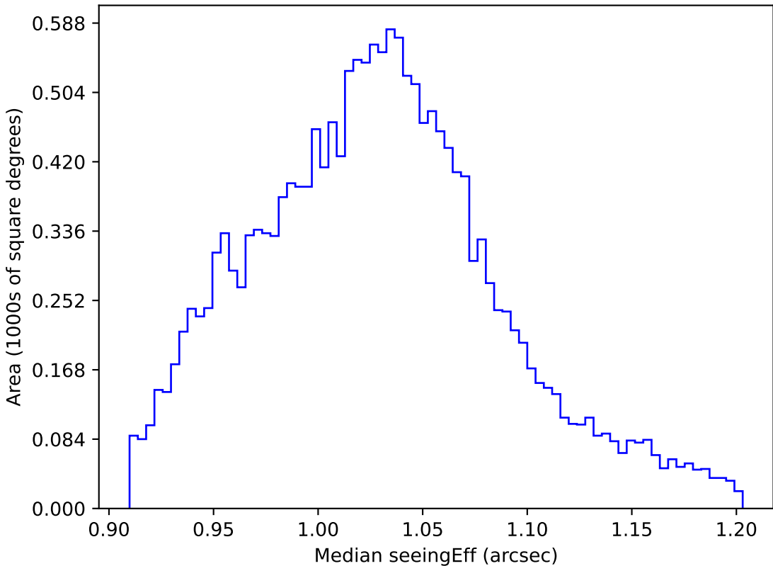
weather_cloudso10v3.4_10yrs WFD y band: Median seeingEff
