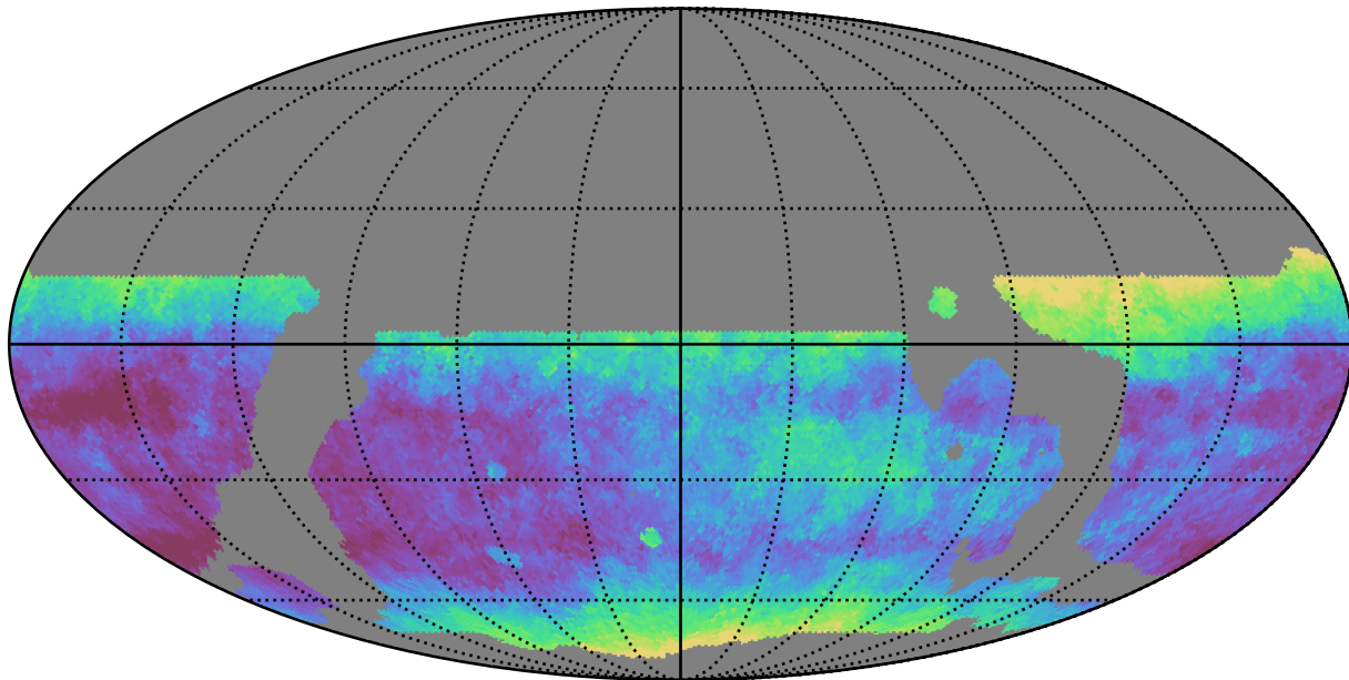
weather_cloudso10v3.4_10yrs WFD r band: Median seeingEff
