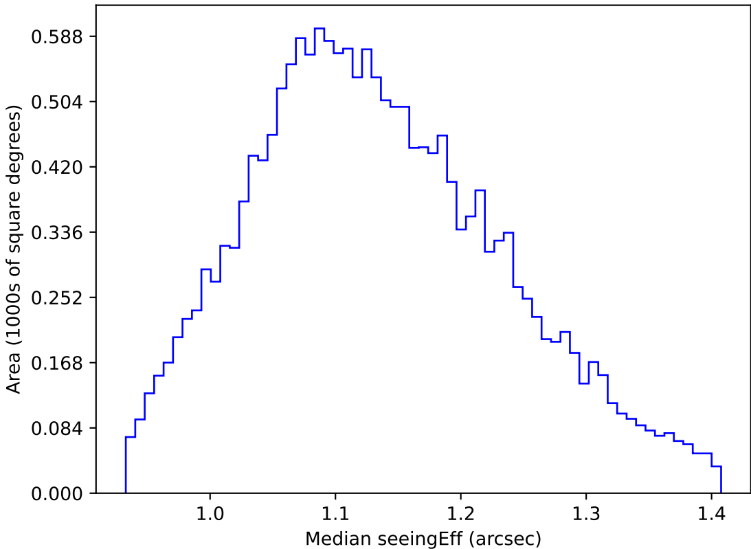
weather_cloudso10v3.4_10yrs WFD g band: Median seeingEff
