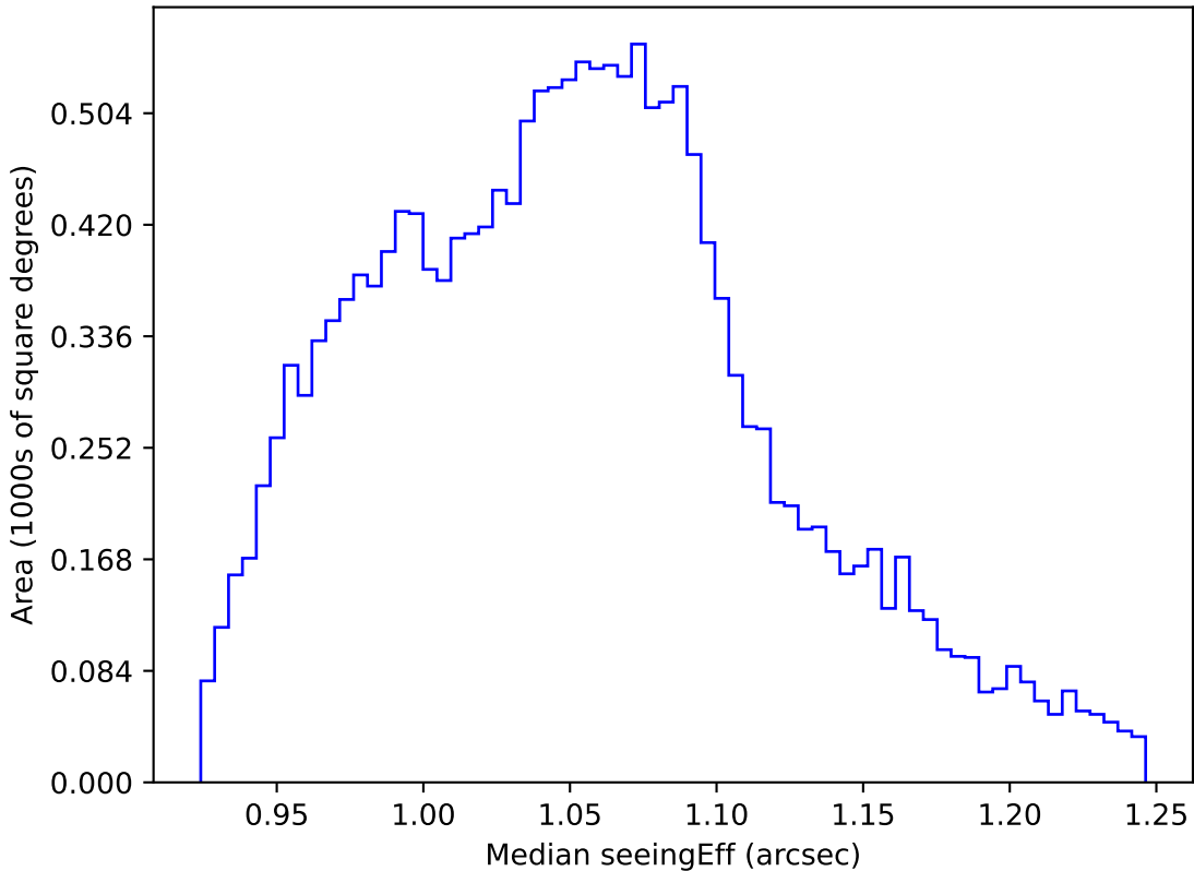
weather_cloudso10v3.4_10yrs WFD all bands: Median seeingEff
