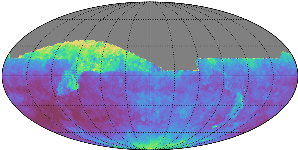
weather_cloudso10v3.4_10yrs All sky z band: Median seeingEff
