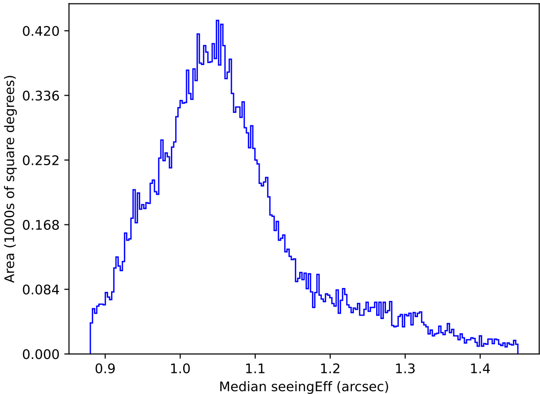
weather_cloudso10v3.4_10yrs All sky z band: Median seeingEff
