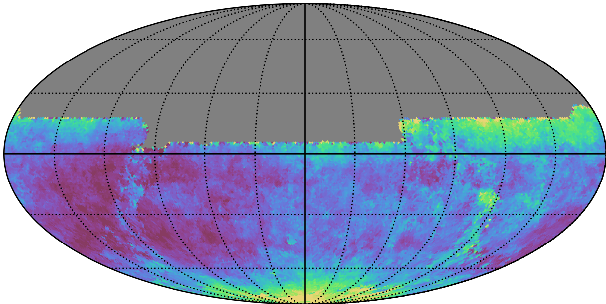
weather_cloudso10v3.4_10yrs All sky y band: Median seeingEff
