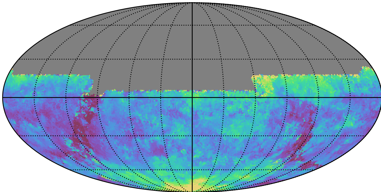
weather_cloudso10v3.4_10yrs All sky u band: Median seeingEff
