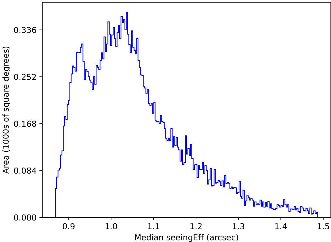
weather_cloudso10v3.4_10yrs All sky i band: Median seeingEff
