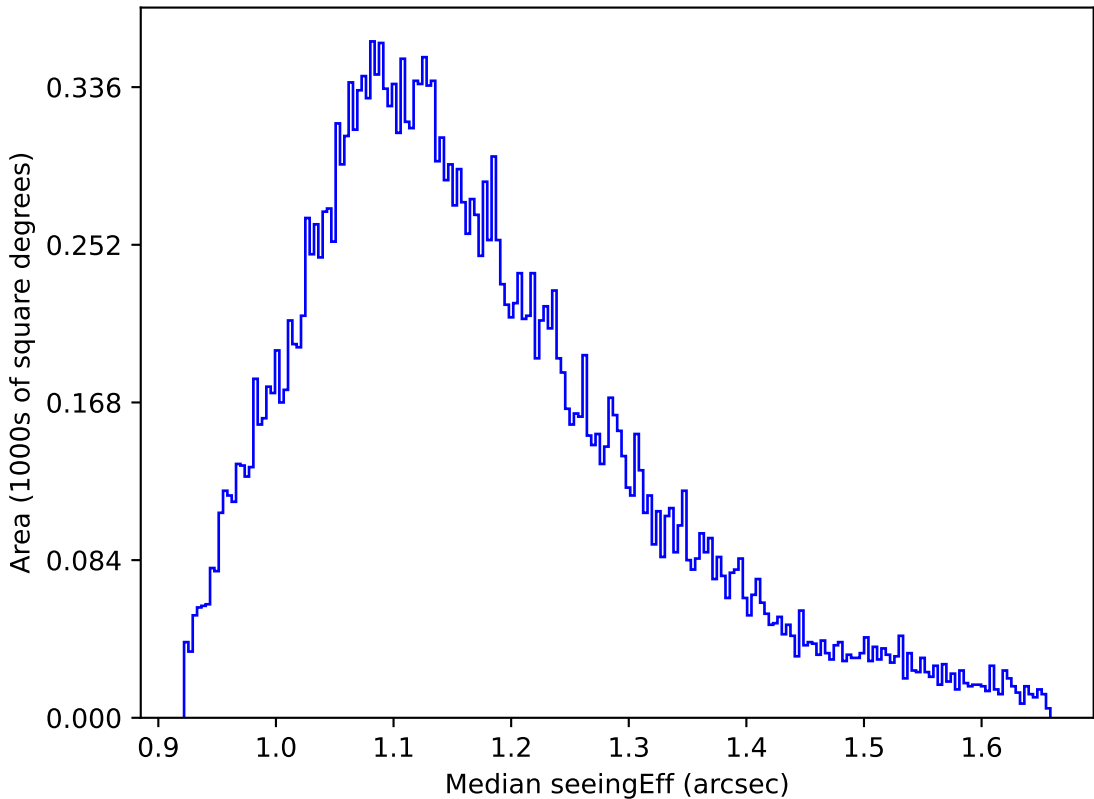
weather_cloudso10v3.4_10yrs All sky g band: Median seeingEff
