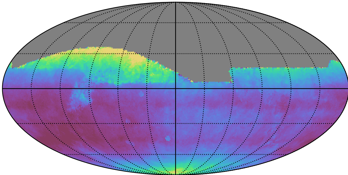
weather_cloudso10v3.4_10yrs All sky all bands: Median seeingEff
