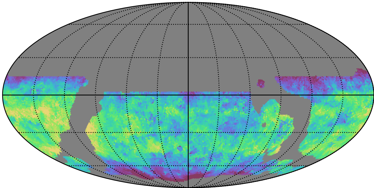
weather_cloudso10v3.4_10yrs WFD u band: Median saturation_mag
