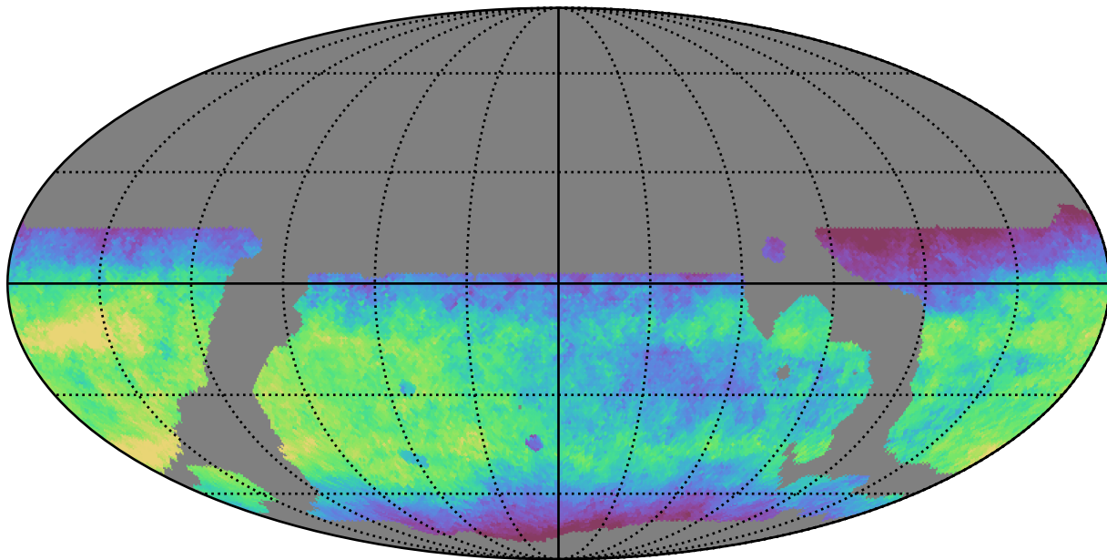
weather_cloudso10v3.4_10yrs WFD r band: Median saturation_mag
