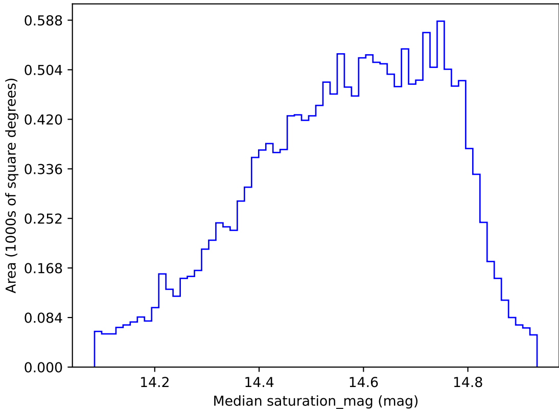
weather_cloudso10v3.4_10yrs WFD r band: Median saturation_mag
