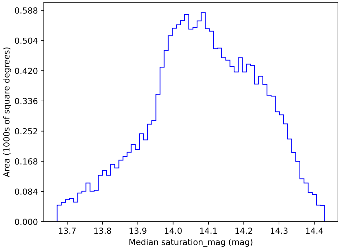
weather_cloudso10v3.4_10yrs WFD all bands: Median saturation_mag
