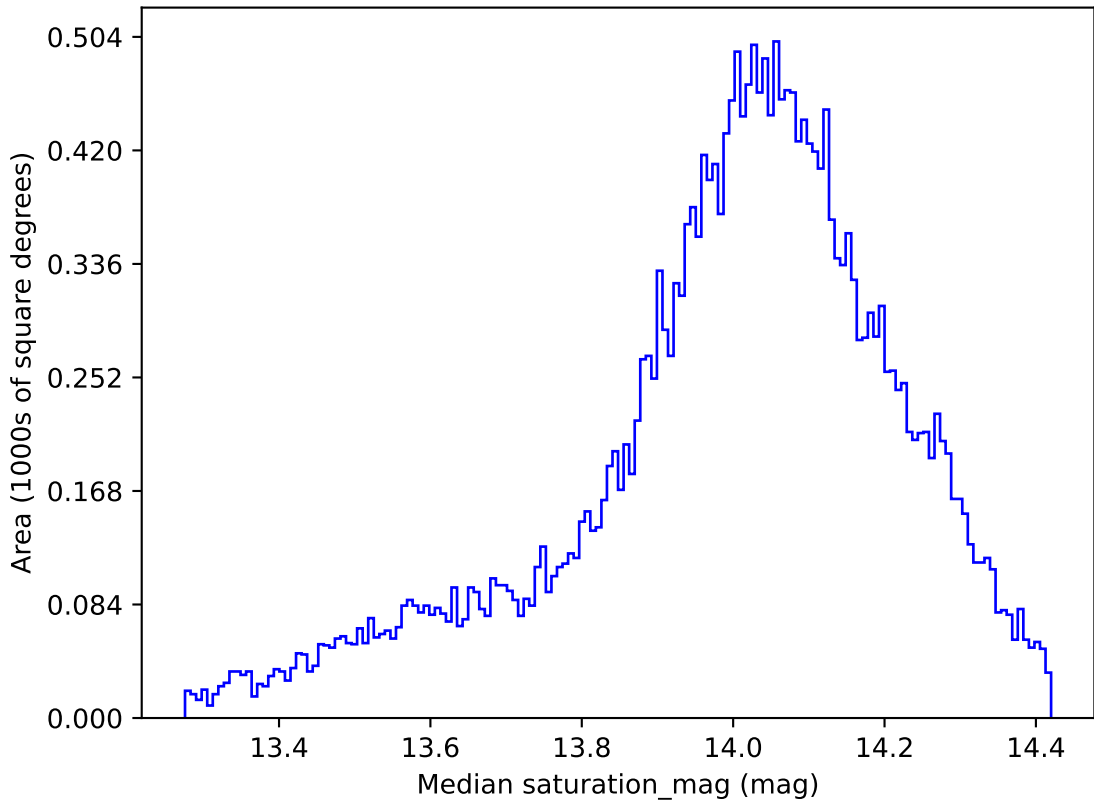
weather_cloudso10v3.4_10yrs All sky z band: Median saturation_mag
