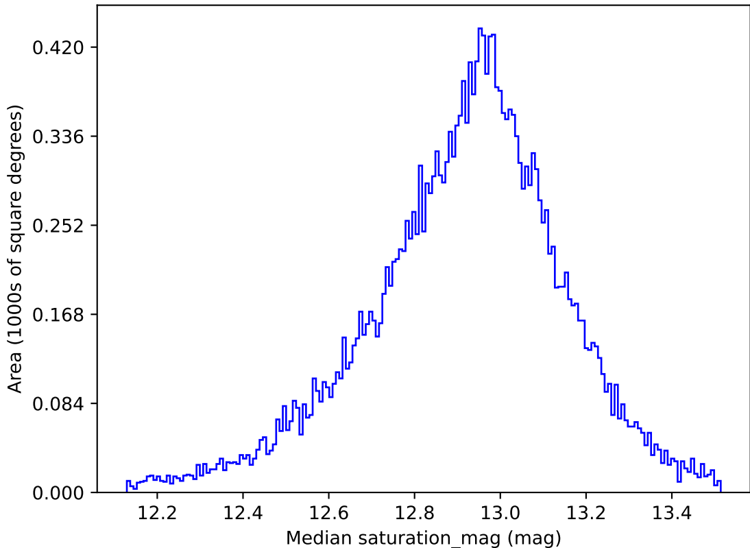
weather_cloudso10v3.4_10yrs All sky u band: Median saturation_mag
