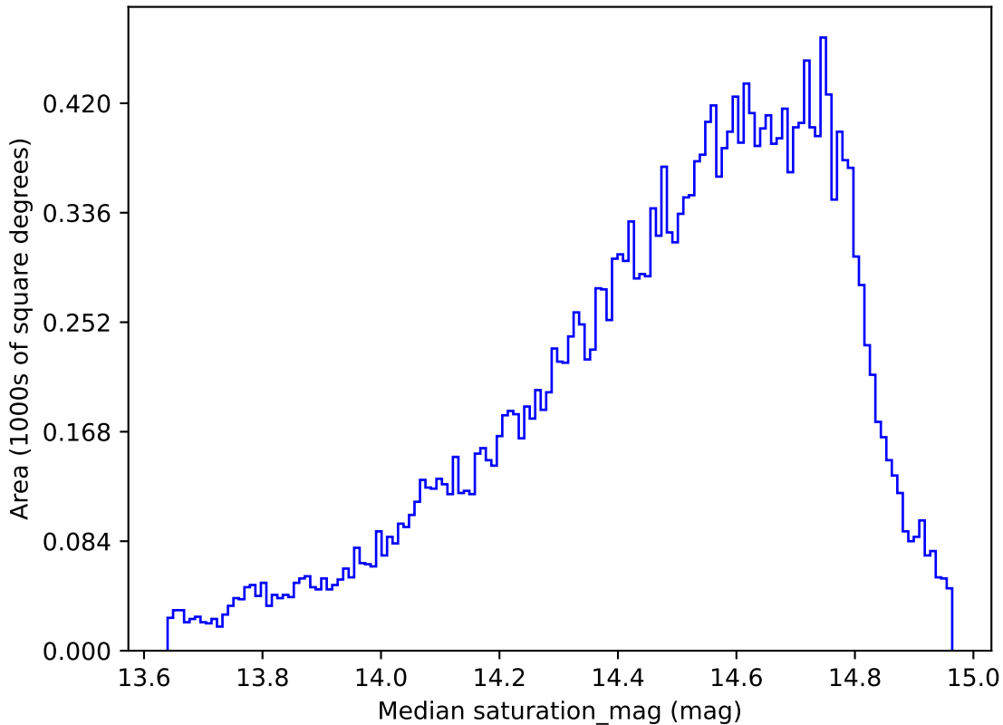
weather_cloudso10v3.4_10yrs All sky r band: Median saturation_mag
