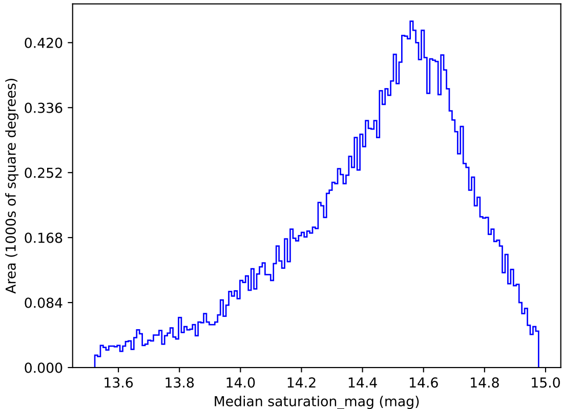
weather_cloudso10v3.4_10yrs All sky g band: Median saturation_mag
