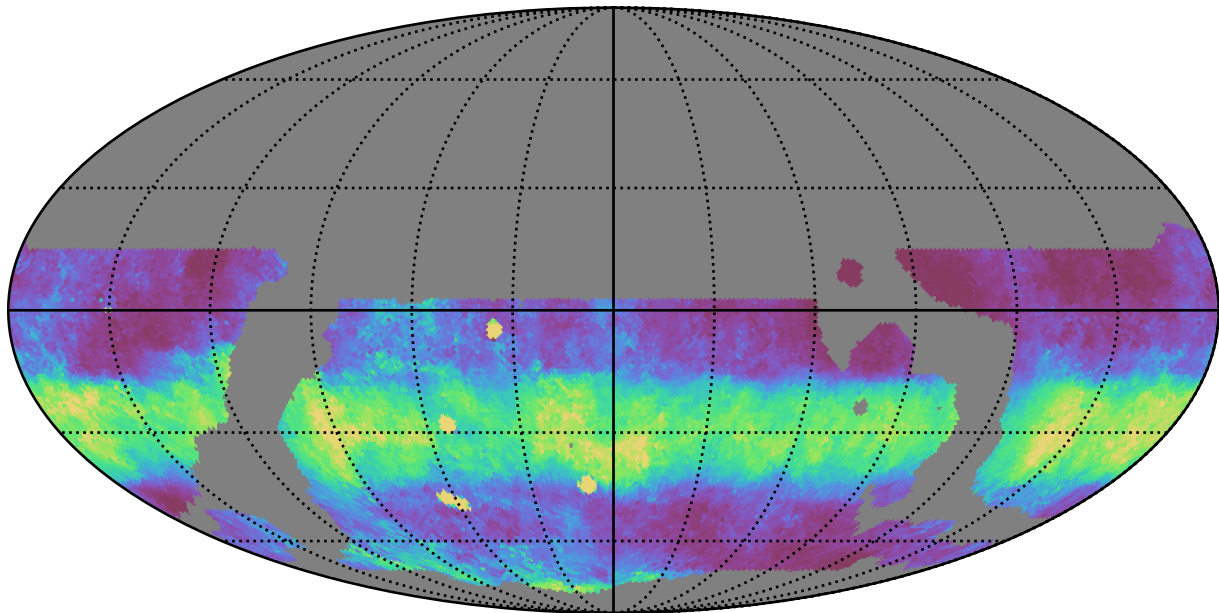
weather_cloudso10v3.4_10yrs WFD z band: Median normairmass
