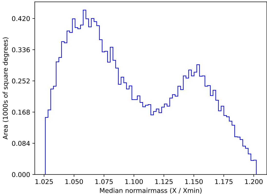
weather_cloudso10v3.4_10yrs WFD z band: Median normairmass
