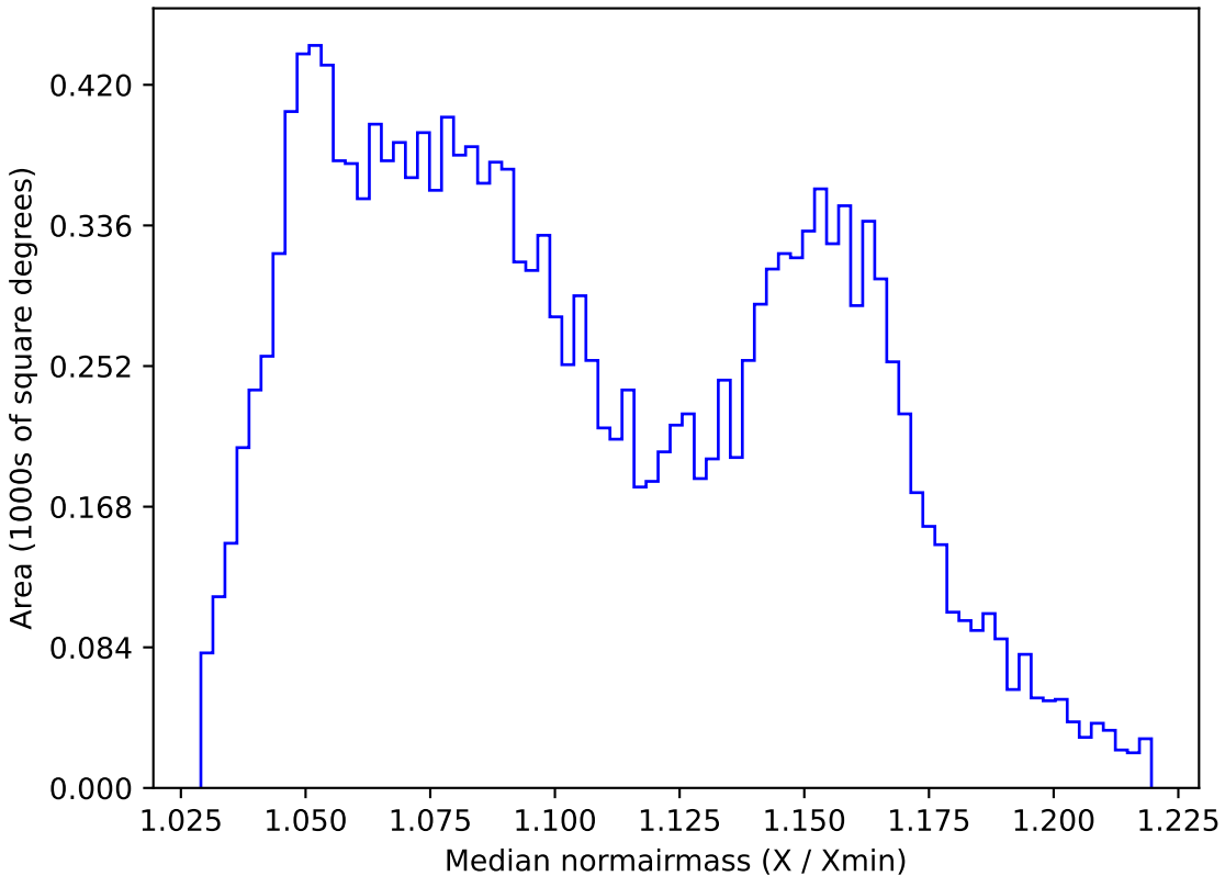
weather_cloudso10v3.4_10yrs WFD y band: Median normairmass
