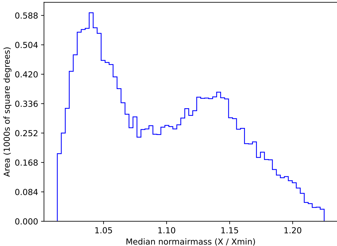
weather_cloudso10v3.4_10yrs WFD u band: Median normairmass
