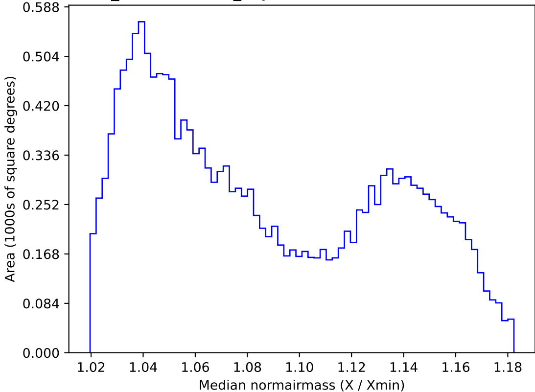
weather_cloudso10v3.4_10yrs WFD r band: Median normairmass
