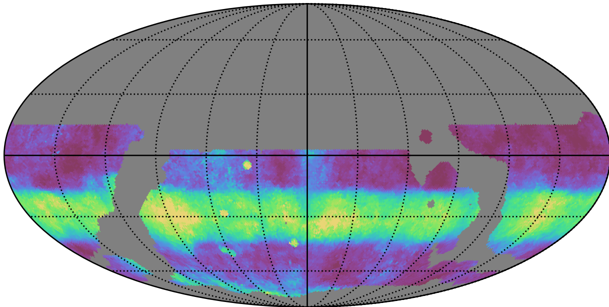
weather_cloudso10v3.4_10yrs WFD i band: Median normairmass
