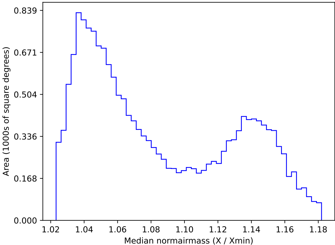
weather_cloudso10v3.4_10yrs WFD i band: Median normairmass
